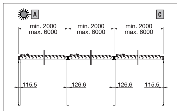
TP6600 Side view of coupled systems
