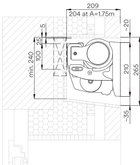
Section of an installation and recess variant, angle of inclination 5° – 10°, rear-ventilated façade
