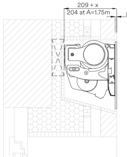
Section of on-site panel installation, angle of inclination 15° – 20°, rear-ventilated façade
