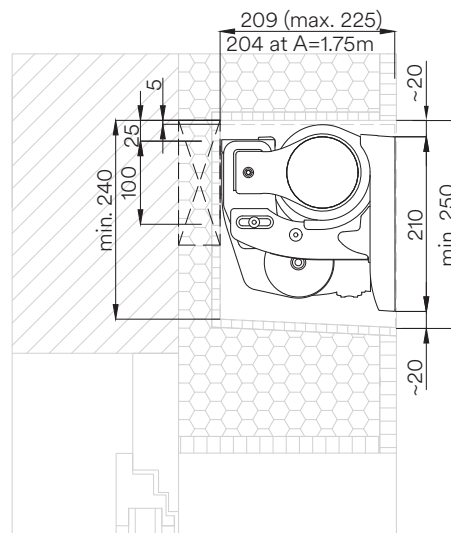
Section of an installation and recess variant, angle of inclination 0° – 5°, plastered façade
