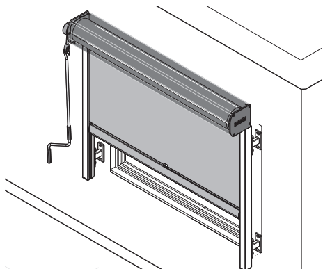
Fig. 9: Manual crank
