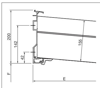
Wall connection
